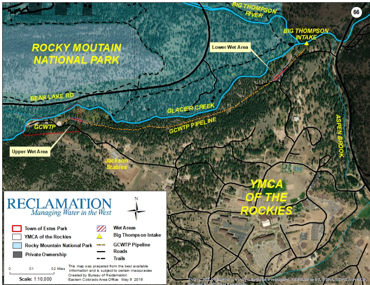
Figure 3-GCWTP Pipeline Alignment
